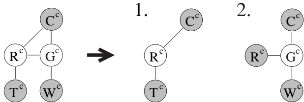
Figure 2. (left) A Comraf model for simultaneously clustering images G^c and their rectangular regions R^c , while taking into account words W^c from image captions, colors C^c and texture data T^c ; (right) a translation of this model into a two-step Comraf*: the first Comraf* is for clustering regions into blobs, whereas the second Comraf* is for clustering images based on these blobs.
